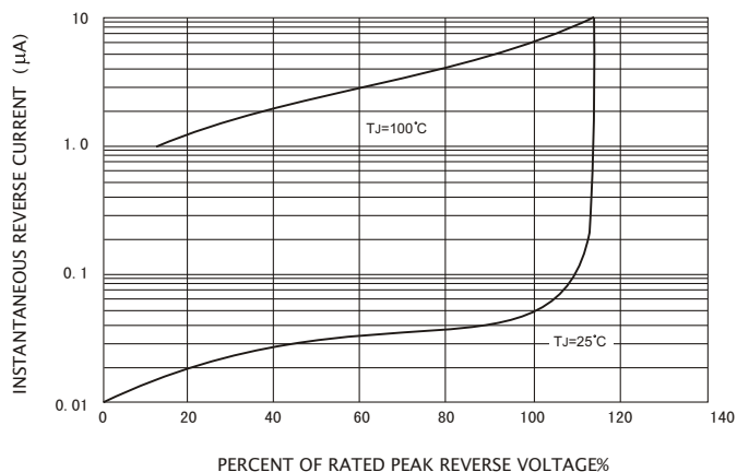
FIG.4-TYPICAL REVERSE CHARACTERISTICS
